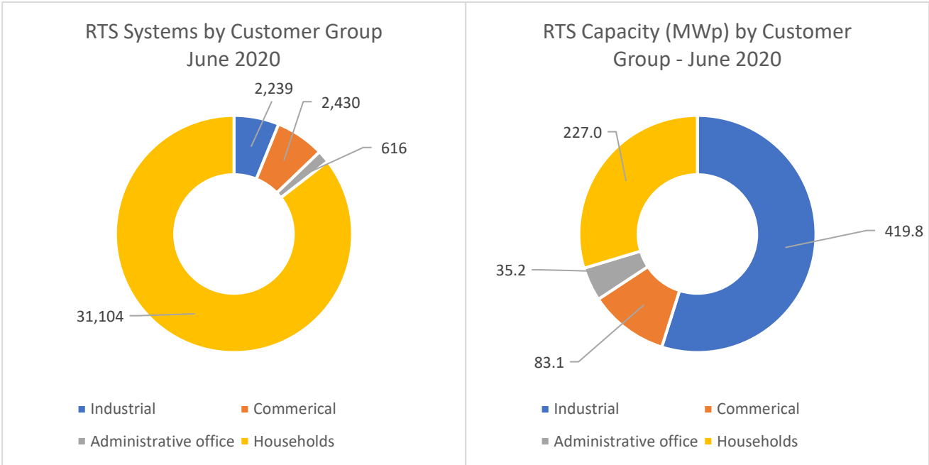
Figure 7. Breakdown of RTS systems and installed capacity by customer group – June 2020
