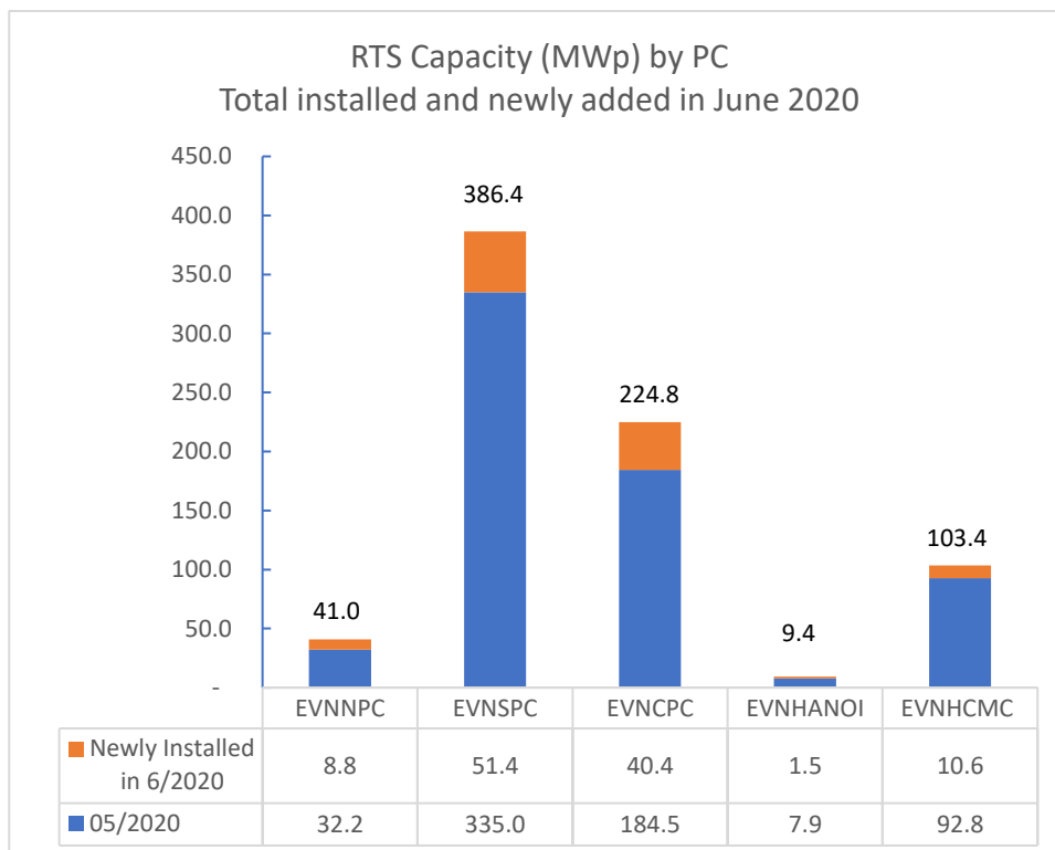
Figure 4. Installed RTS capacity (MWp) by PC - in June 2020
