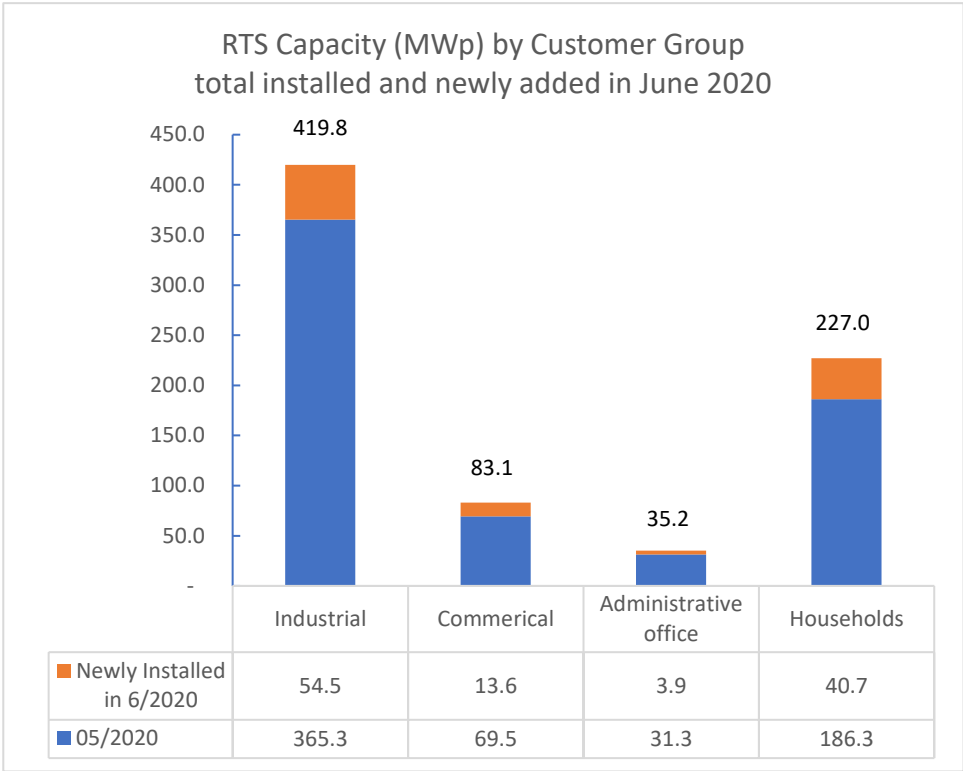
Figure 8. Total installed capacity by customer group (MWp) – June 2020
