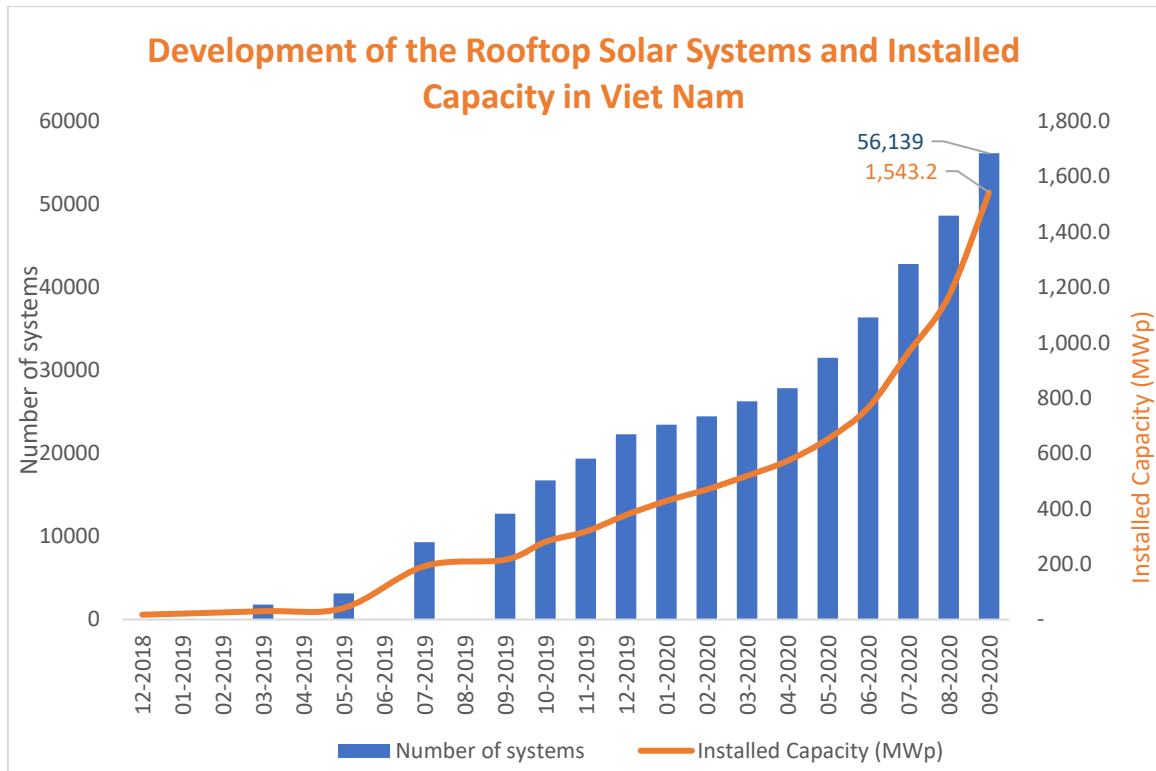
Figure 1. Total RTS systems and installed capacity (MWp) in Viet Nam by the end of September 2020
