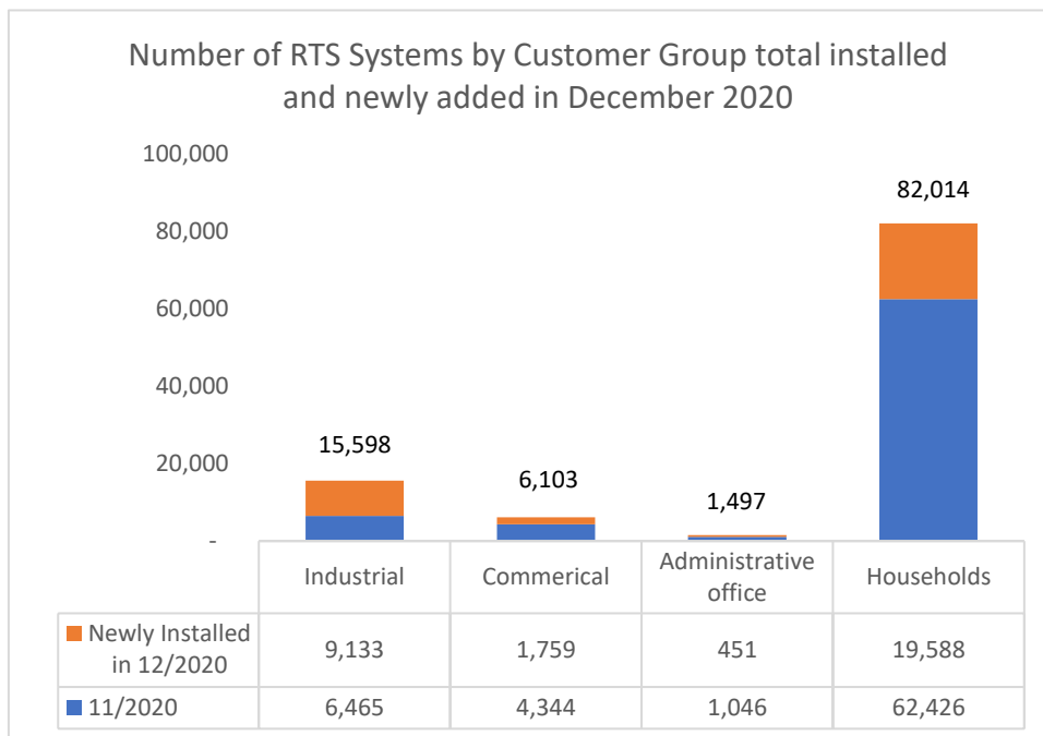
Figure 6. Number of RTS systems by customer group – December 2020
