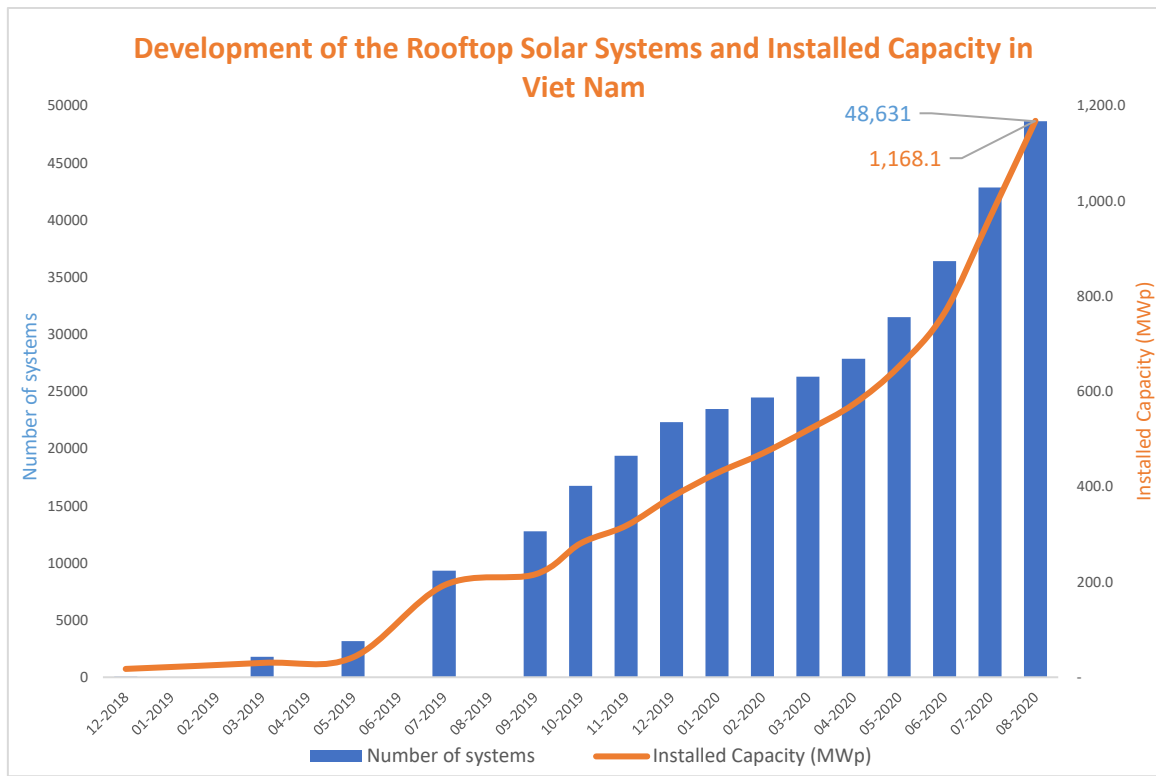
Figure 1. Total RTS systems and installed capacity (MWp) in Viet Nam by the end of August 2020
