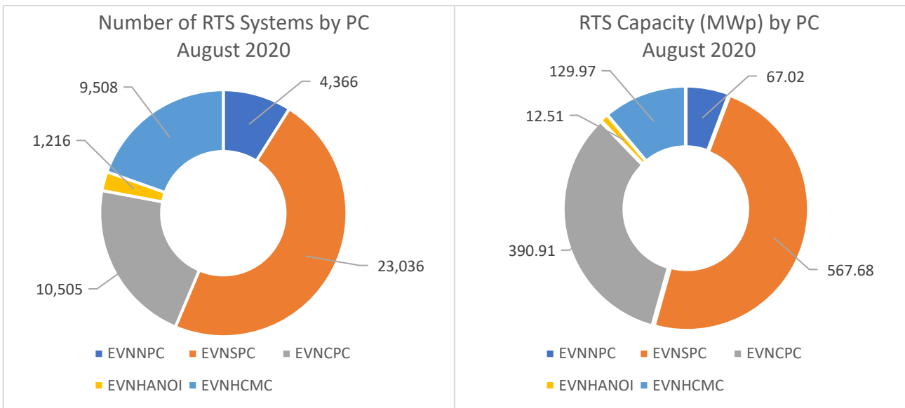
Figure 5. Break down of number of RTS systems and installed capacity by PC – August 2020
