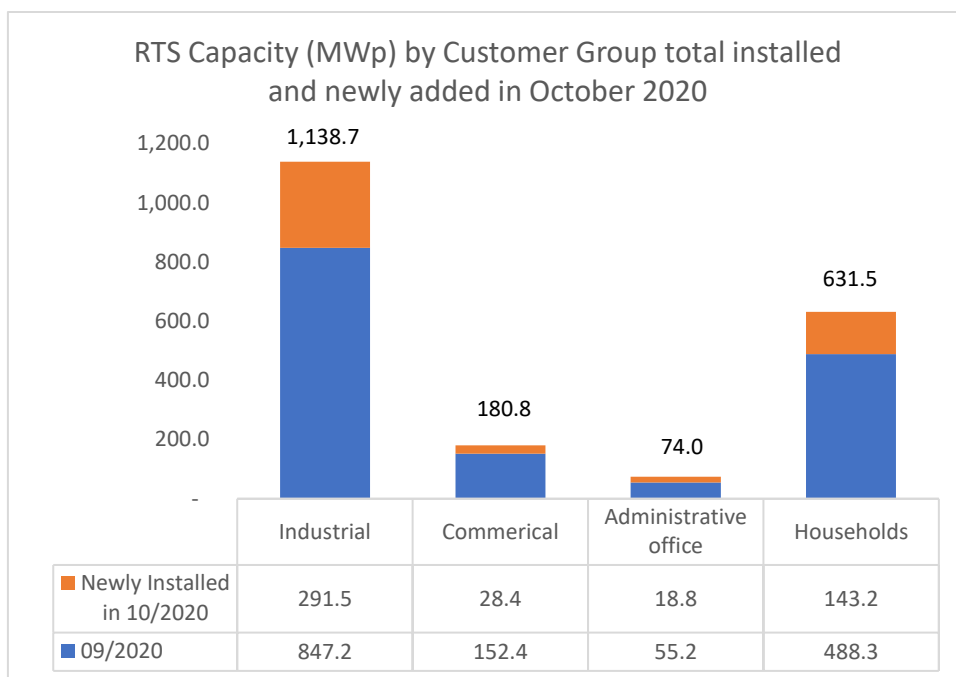
Figure 7. Total installed capacity by customer group (MWp) – October 2020
