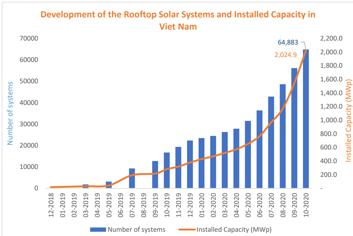
Figure 1. Total RTS systems and installed capacity (MWp) in Viet Nam by the end of October 2020
