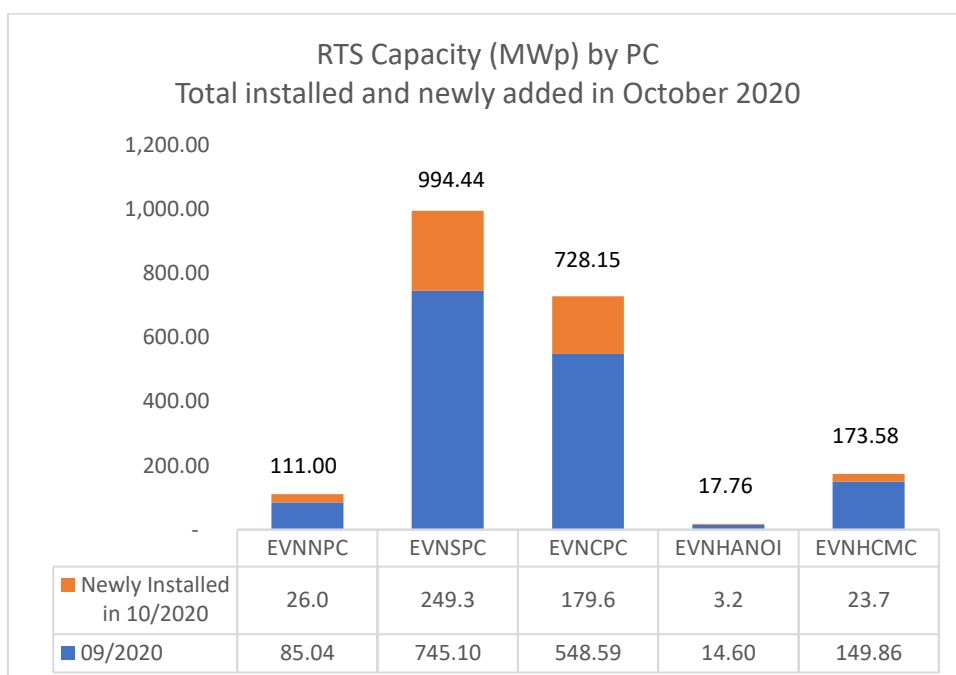
Figure 4. Installed RTS capacity (MWp) by PC - in October 2020
