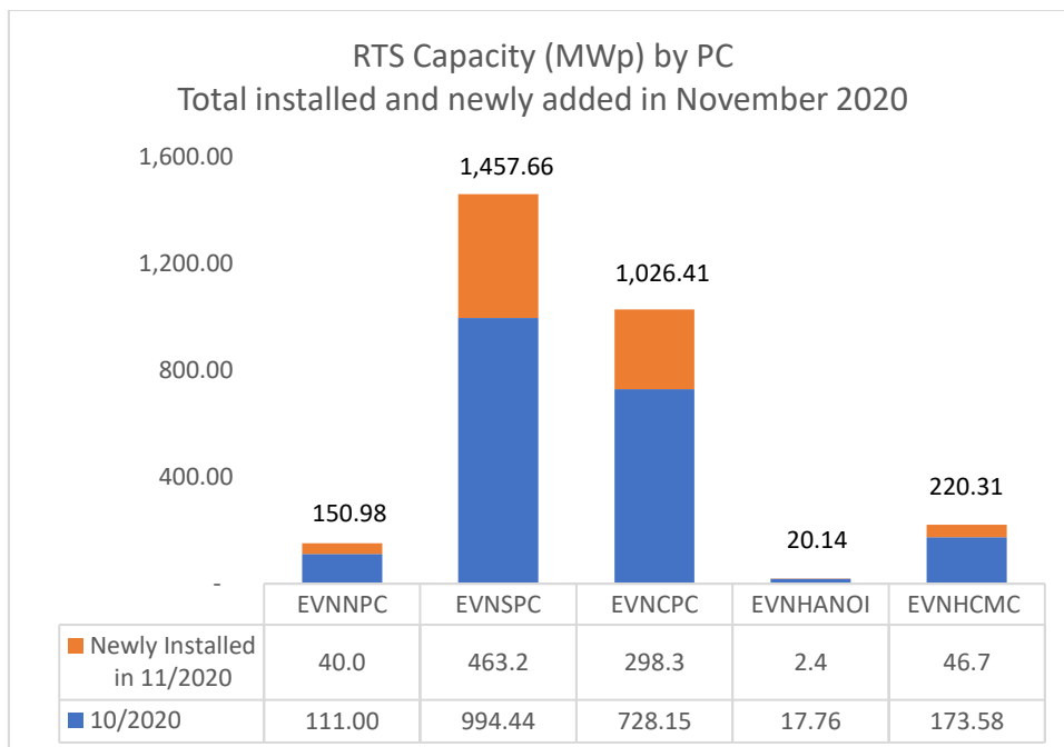
Figure 4. Installed RTS capacity (MWp) by PC - in November 2020
