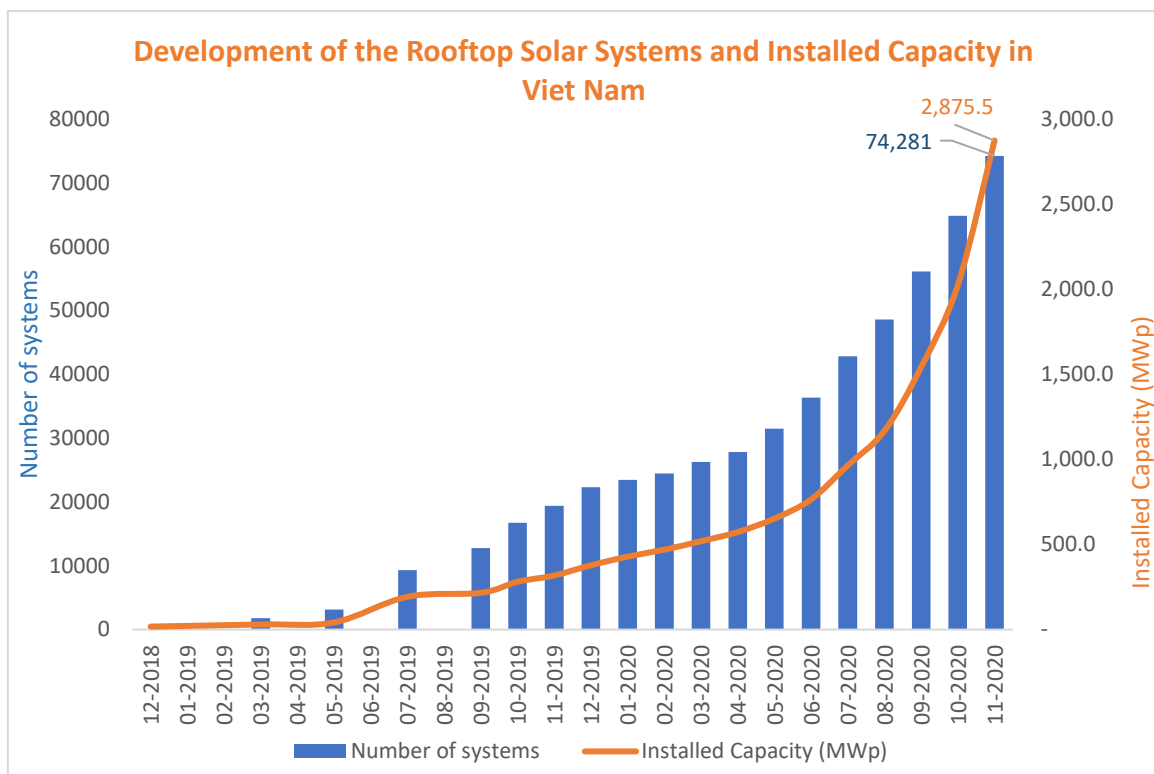
Figure 1. Total RTS systems and installed capacity (MWp) in Viet Nam by the end of November 2020
